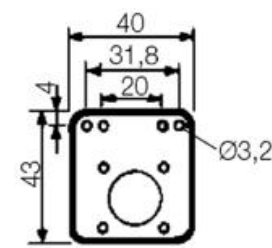
Monteringsplatta 6050-6000-6001
