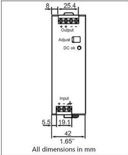
Fig. 20-1 Front view
