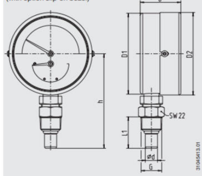
Model 100.10.80, lower mount (LM) (with option slip-on bezel)
