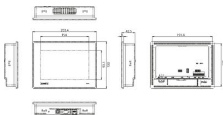
Panel Cut Out Dimensions: 192 x 138.5 mm (7.56" x 5.45")
