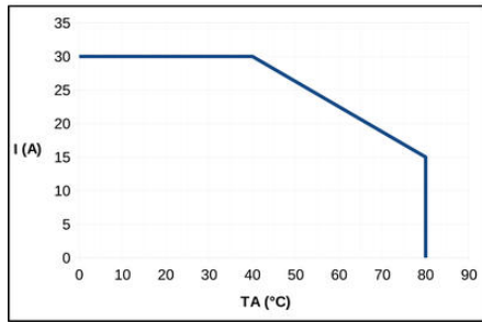
DERATING CURVES
