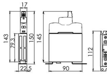
DIMENSIONS (mm)
