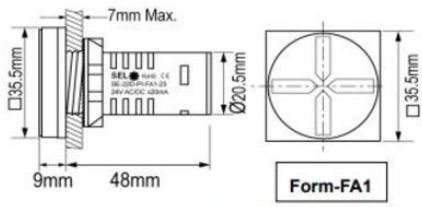
Outline Dimension
