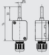
Model TF41 with probe sleeve
